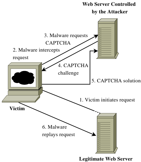
Figure 1: CAPTCHA Smuggling
